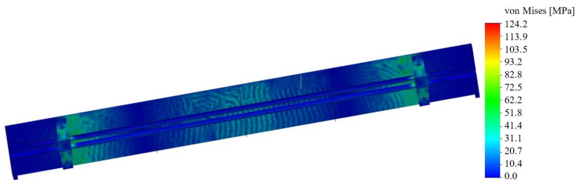
Figure 9. A stress state of the passenger car frame with the adapter
