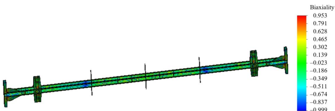
Figure 6. The passenger car frame biaxiality indicator
