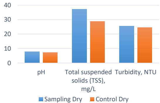
Figure 3. Average pH, total suspended solids, and turbidity from sampling areas compared to control areas during the dry season.
