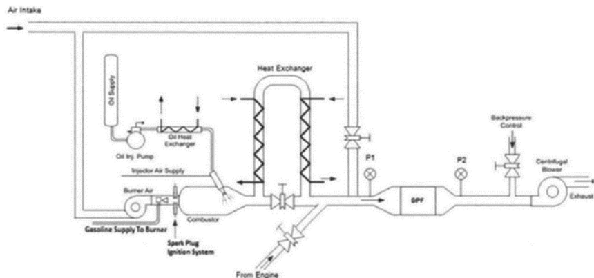
Figure 3. GPF aging system [18]
