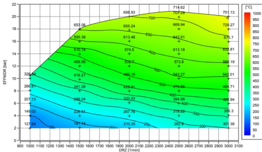
Figure 1. GPF temperature change map
