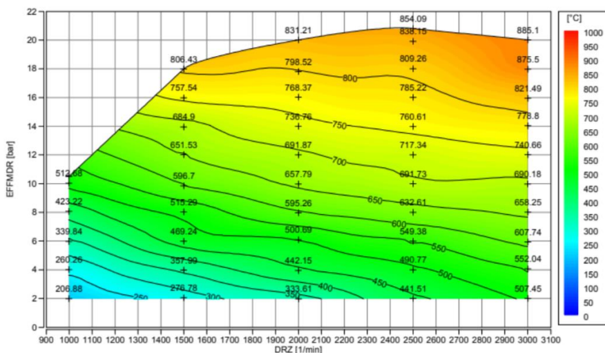
Figure 2. Catalyst temperature change map
