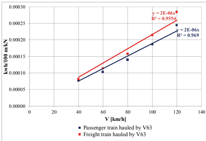
Figure 9. Specified energy consumption of V63 locomotive
